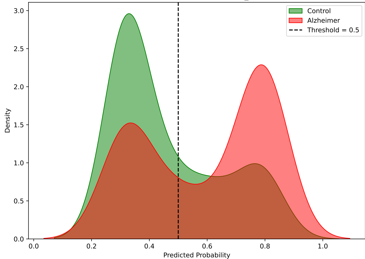
Risk Score Distribution - SVM_RBF
